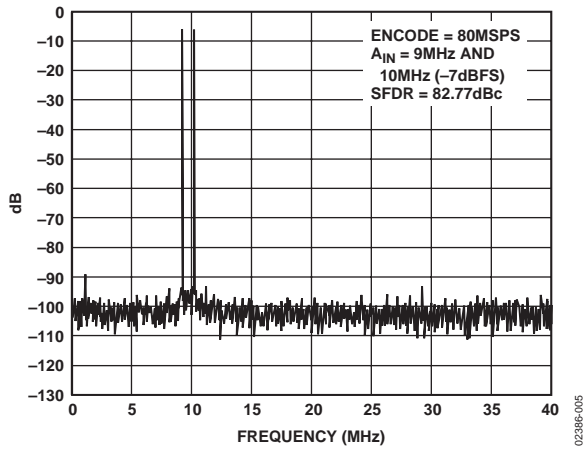
Figure 6. Two Tone @ 9 MHz/10 MHz
