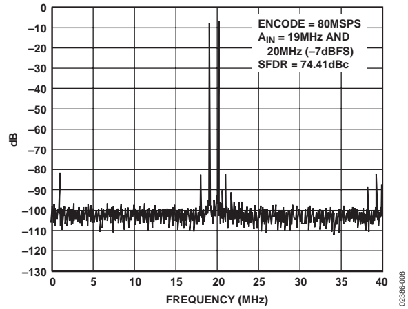
Figure 9. Two Tone @ 19 MHz/20 MHz
