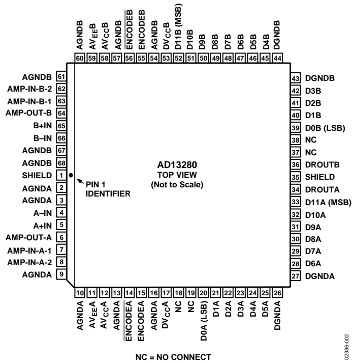
Figure 3. Pin Configuration
