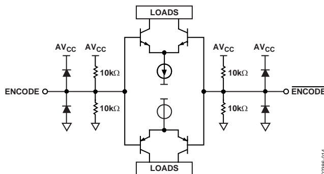
Figure 15. ENCODE Inputs
