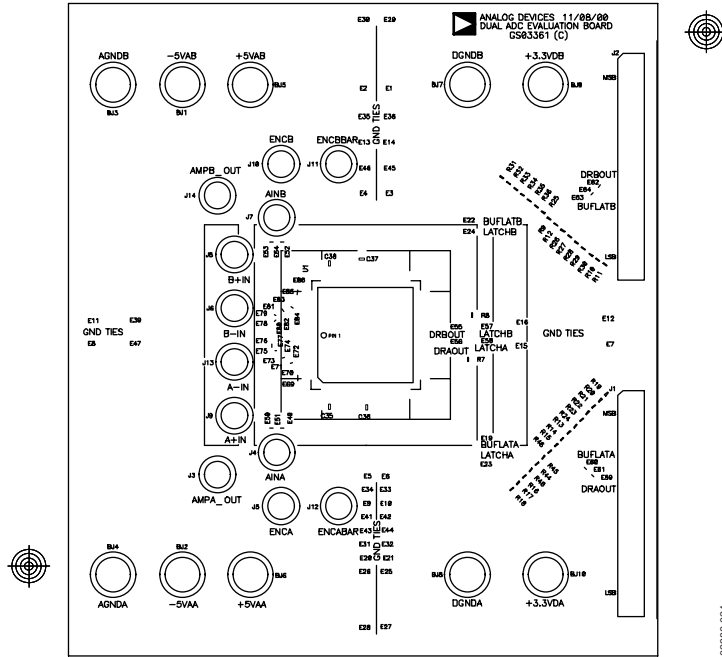
Figure 24. Top Silk
