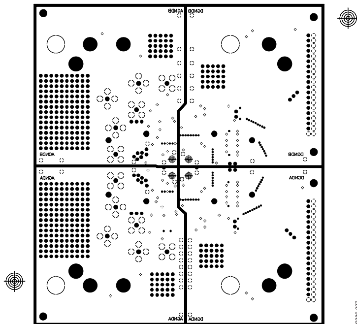
Figure 27. GND2
