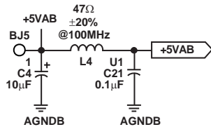
Figure 21. Evaluation Board
