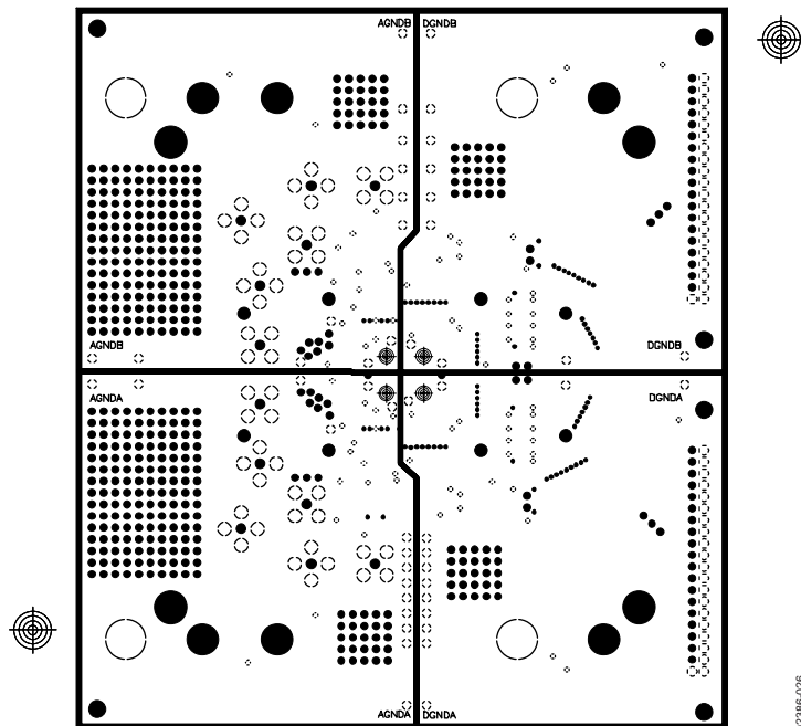
Figure 26. GND1
