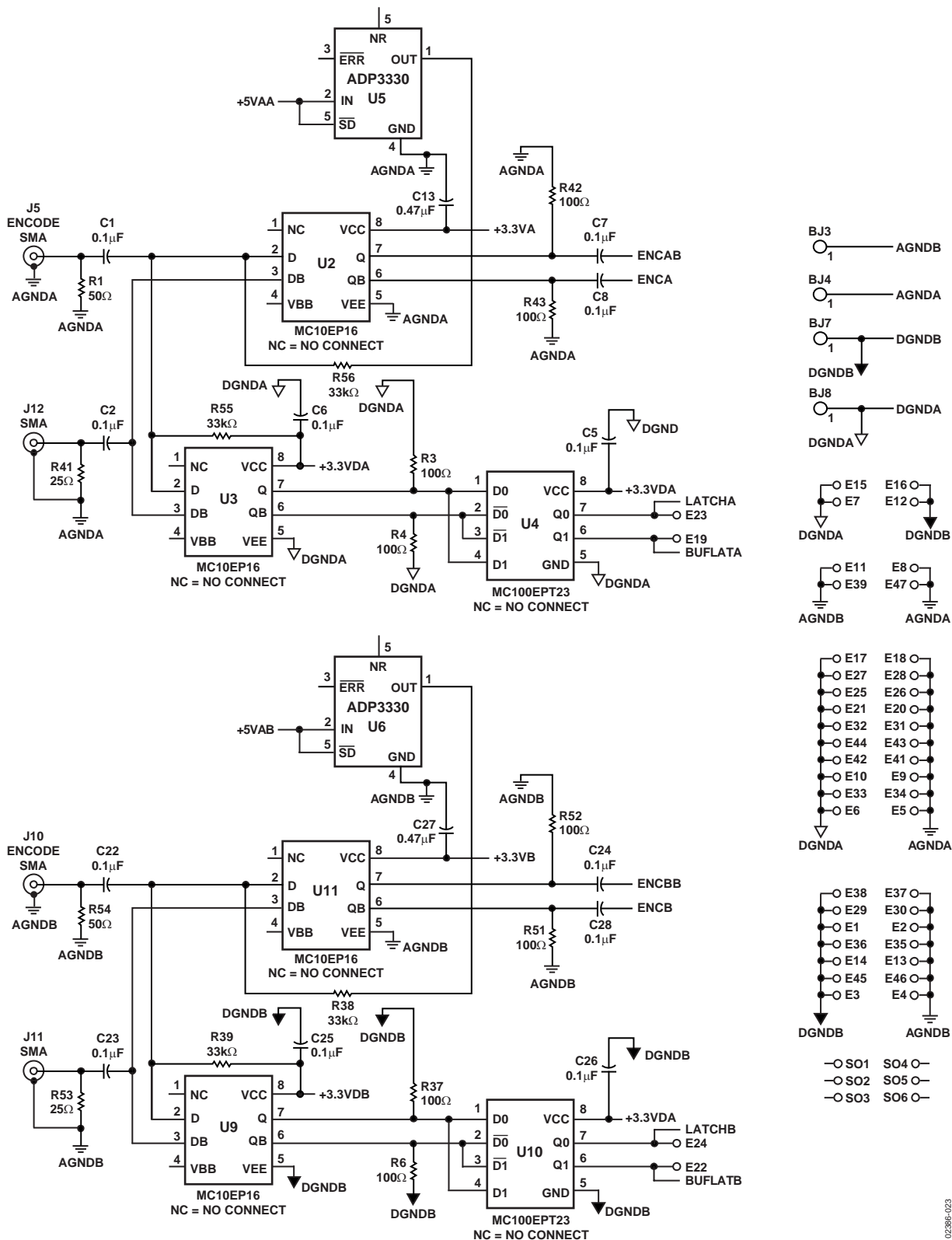
Figure 23. Evaluation Board
