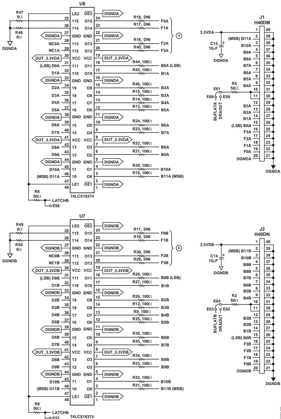
Figure 22. Evaluation Board
